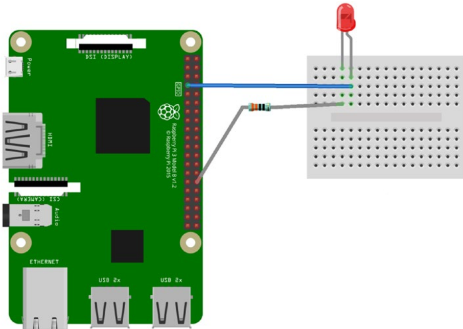
Figure 21-18. The circuit for the Python controlled LED
