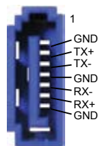
SATA_1/2/3/4
